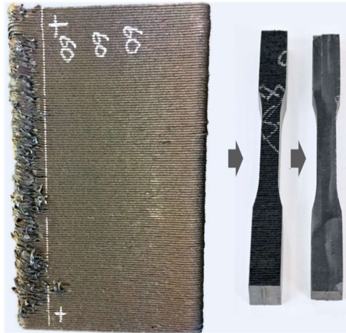
measuring the width and thickness in three locations using a caliper (Mitutoyo, Japan). A UH-F300kNX universal testing machine (Shimadzu Corp., Japan) was used to test the samples, using a strain rate of 5 mm/min. Figure 3.9 Four tensile bars are waterjet cut from each 3D printed slab then machined.
