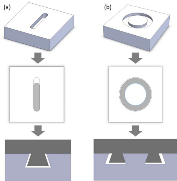
Figure 3.4 a) Open-ended versus b) closed-loop contour for dovetail feature.
