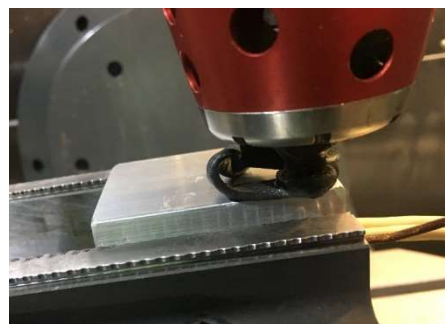
Figure 3.1 Extruded polymer fails to adhere to a clean aluminum surface.
